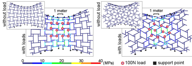
Figure 16: von Mises stress plots. The colors indicate the amount of stress on the rods; note the maximum stress for bamboo and pine wood are around 350\text{MPa} and 40\text{MPa} , respectively.
