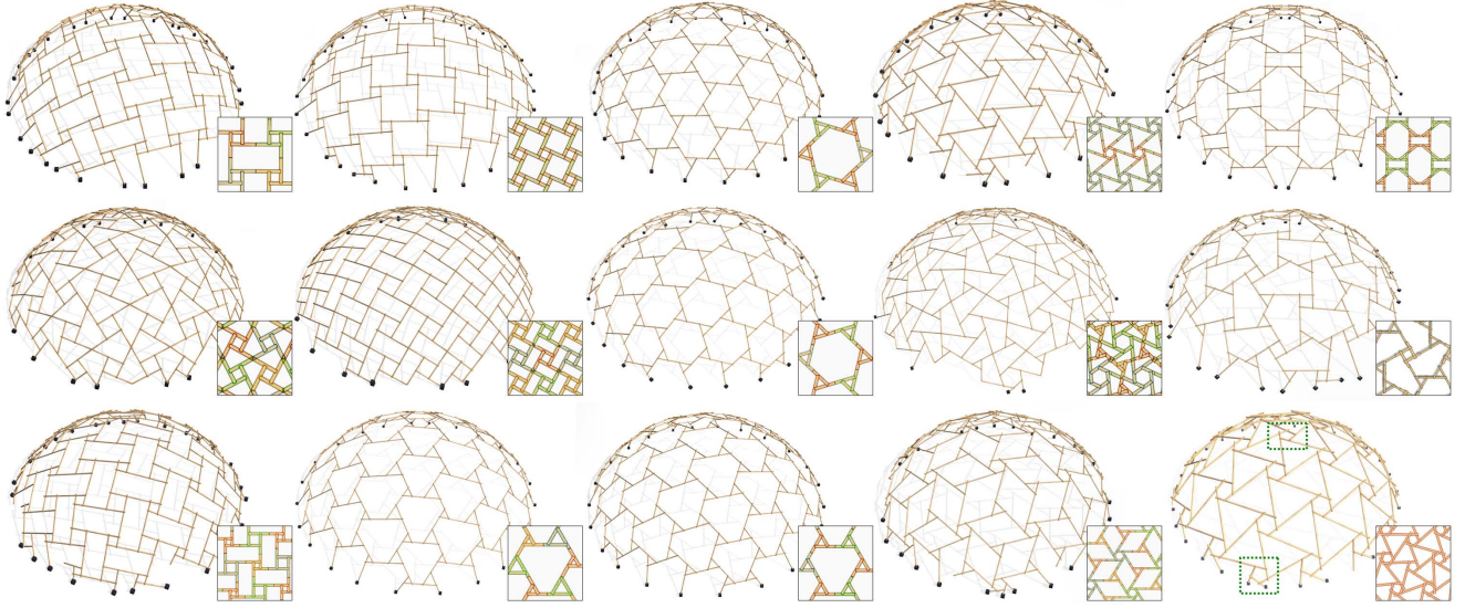
Figure 15: Our tool supports a wide variety of RF-tessellation patterns for designing RF-structures of different appearance.
