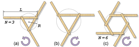
Figure 5: (a) parameter labels on an N = 3 counter-clockwise RF-unit. (b) a clockwise RF-unit with a larger R and L . (c) an N = 6 clockwise RF-unit. Note: all rods are on top of others.
