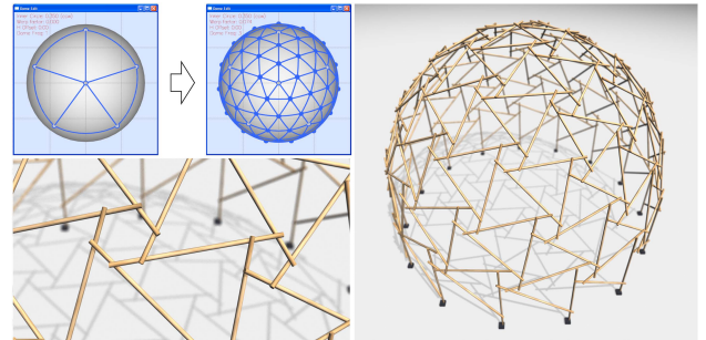
Figure 19: The Da Vinci dome designed by our tool.
