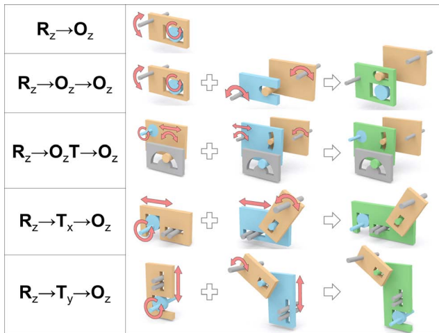
Fig. 9. All possible motion transfer chains with two or fewer eleMechs for achieving R_z \rightarrow O_z (the axis-aligned target motion).
