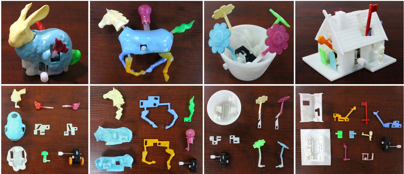
Fig. 18. Four of the six wind-up toys (top) that we have fabricated and assembled from 3D-printed parts (bottom). From left to right: BUNNY (13.0g shell + 7.8g motor + 9.0g mechanism), HORSE (15.3g shell + 5.9g motor + 26.1g mechanism), FLOWER POT (34.8g shell + 5.8g motor + 8.0g mechanism), and HOUSE (48.9g shell + 6.0g motor + 6.4g mechanism). See their statistics in Table 3.
