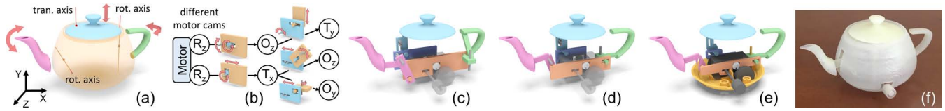
Fig. 3. Overview of our system. (a) Segmented TEAPOT model (i.e., body, handle, spout, and lid) with user-provided motion on each end-effector part (motion arrows and axes colored in red); (b) our system first constructs motion transfer trees to guide the selection of elemental mechanisms; (c) then, it orientates and connects elemental mechanisms to form an initial wind-up mechanism, (d) optimizes the joints and parts in each elemental mechanism with a kinematic analysis, subject to fabrication and collision constraints, and (e) post-processes the toy to refine parts boundary shape, and create the body shell and support structures for fabrication. (f) The 3D-printed wind-up toy result.
