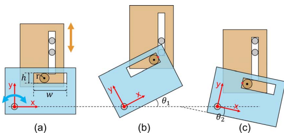
Fig. 7. Given the target motion range ( \theta_1 and \theta_2 in (b & c)) of the driver, a predefined value for r in (a), and the joint layout \{J_{layout}\} , we can derive the joint geometry \{J_{joint}\} of this driver-follower joint accordingly, i.e., h and w in (a). Please refer to the supplemental material for details.
