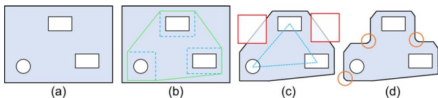
Fig. 17. Procedure to refine the boundary shape of mechanical parts: (a) given joints on major plane; (b) we compute a convex hull (in green) that encloses the joints with a small margin (in blue); (c) we then identify structural lines (in blue) in-between joints and crop the convex hull without cutting through the structural lines (in red); and (d) lastly, we round the corners of the shape (in orange).
