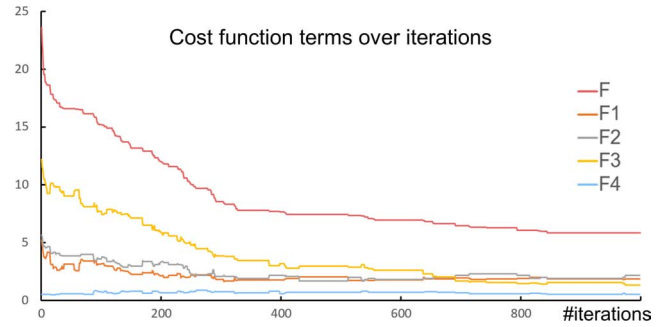
Fig. 15. Plot of cost function over iterations (see Eq. (1)) during the fine optimization process, for BUNNY shown in Fig. 12(d).
