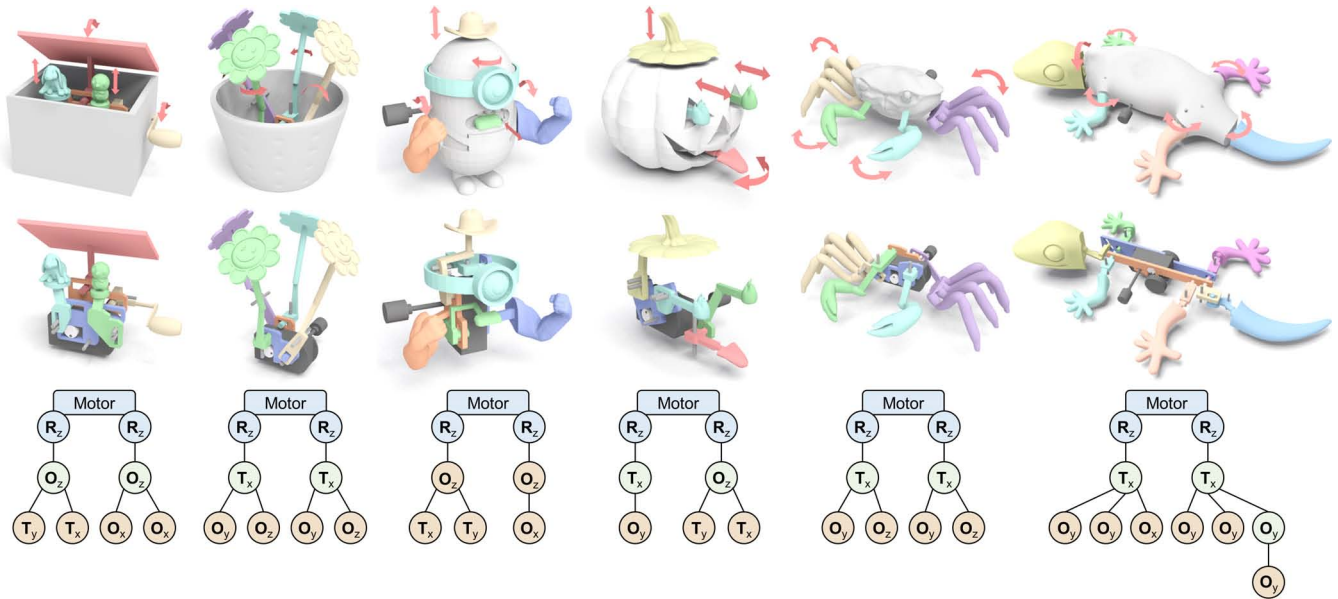
Fig. 16. Wind-up toys designed by the participants in the user evaluation and generated from our system accordingly; from left to right: Box, FLOWER POT, MINION, JACK O’LANTERN, CRAB, and GECKO. From top to bottom: input models and user-prescribed toy part motions, the optimized wind-up mechanisms, and the associated motion transfer trees.
