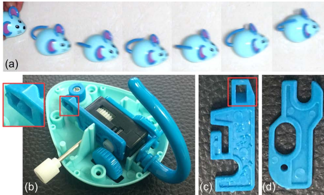
Fig. 2. An example wind-up toy (see its live motion in supp. video). (a) It moves along a curved path while swinging its tail; (b) the internal wind-up mechanism and motor; and (c&d) nontrivial parts for motion transfer, e.g., from a continuous rotation (spring motor) to a periodic swing (tail).
