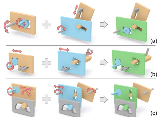
Fig. 8. Different cases of connecting two eleMechs (based on the type of supporters), we merge the follower of the parent (left) with the driver of the child (middle) into a single part in green (right).
