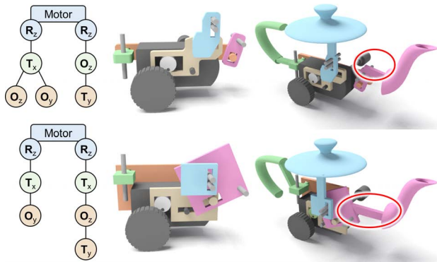
Fig. 19. Comparing mechanisms produced from our system (top) and from the baseline method (bottom). Although both results are functional, our optimized TEAPOT has shorter kinematic chains (top left), a more compact mechanism with smaller mechanical parts (top middle), and shorter connectors to join the end effectors with external parts (see the red circles).
