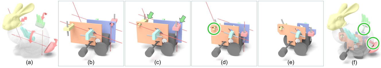
Fig. 12. (a) Inputs; (b) initial mechanism; (c) coarsely-optimized mechanism, where some parts relocate to different sides (see green arrows); (d) finely-optimized mechanism, where some joints (see the green circle) reorientate on the major plane to better match the prescribed motion; (e) boundary shapes of parts are refined; and (f) end-effector parts connect with associated external toy parts (see green circles).
