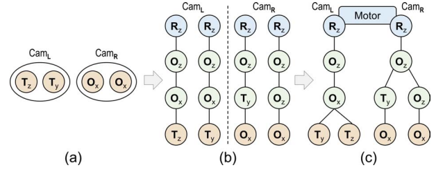
Fig. 10. A typical example: (a) end effectors assigned to left and right cams; (b) kinematic chains picked for each end effector; and (c) chains merged into a motion transfer tree for each cam.
