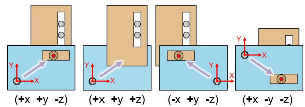
Fig. 13. Four of the eight choices in roughly positioning a driver-follower joint in the local space \mathbb{S}_P of the driver's major plane.
