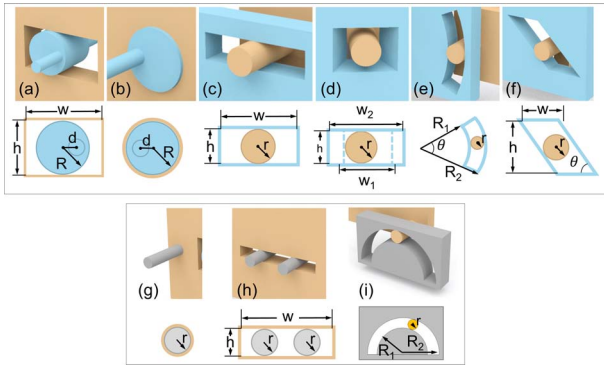
Fig. 6. Driver-follower joints (top) and support joints (bottom) in the eleMechs shown in Fig. 4. All are higher pair joints, except (b) and (g).
