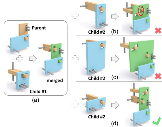
Fig. 11. Connect a parent eleMech to two child eleMechs. We first connect the parent eleMech with (a) child #1 eleMech, and then with (b-d) child #2 eleMech. Three \{J_{layout}\} examples are shown: (b) the merged part is structurally weak (see the red circle), since the joints are too close to one another; (c) the merged part is large and heavy, since the joints are too far from one another; and (d) the merged part in this example is desired.
