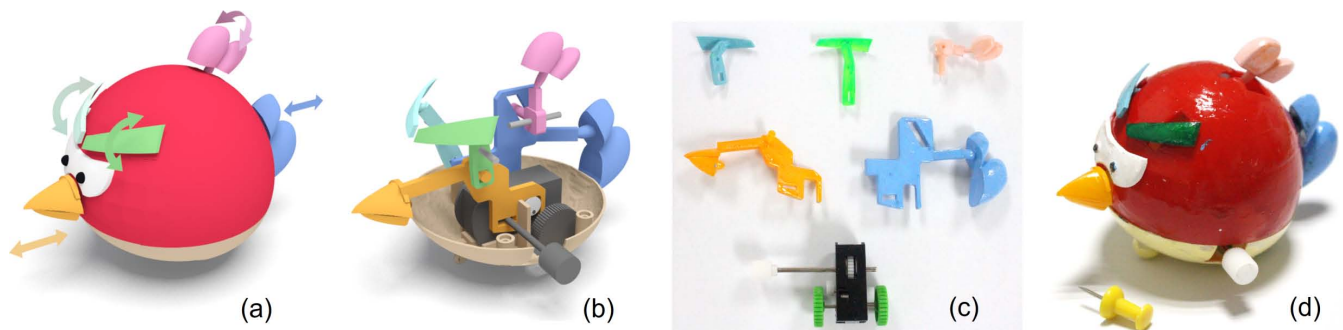
Fig. 1. (a) Input model with user-provided parts geometry and motion; (b) wind-up mechanism constructed by our method; (c) 3D-printed parts (top two rows) and spring motor (bottom); and (d) assembled toy ( 9.2 \times 6.7 \times 6.4 \text{ cm}^3 ; and 16.1g shell + 7.9g motor + 7.3g mechanism).
